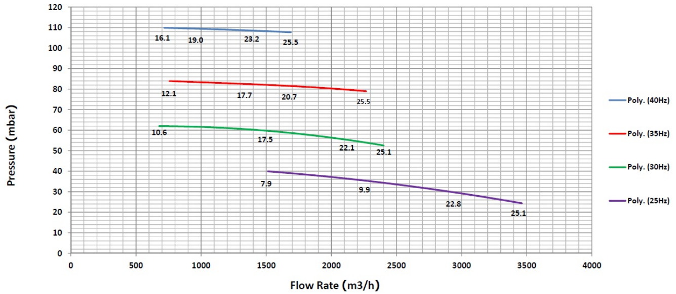
Performance Curve
